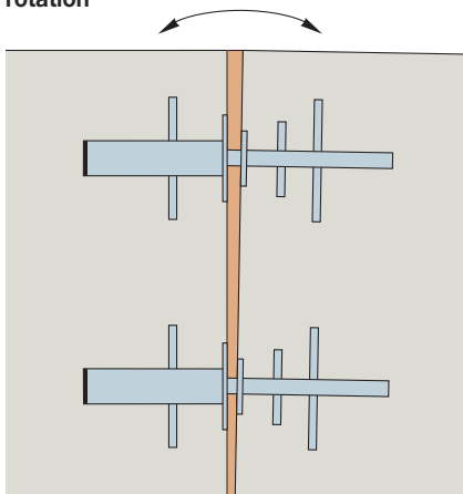
Ancon DSDQ Shear Connectors allowing rotation
